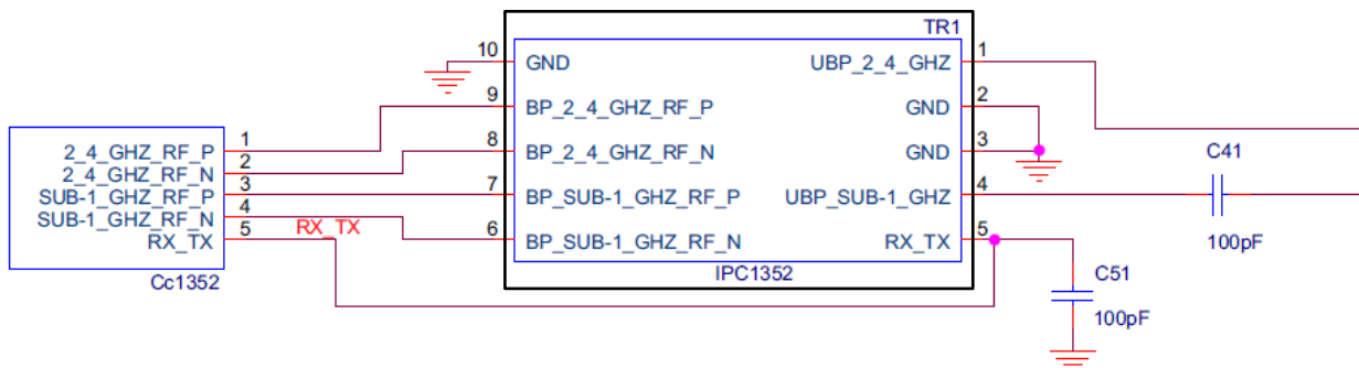
FIGURE 3. IPC REFERENCE DESIGN
